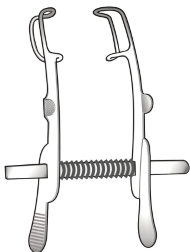
MELLINGER BV 02 70 mm
